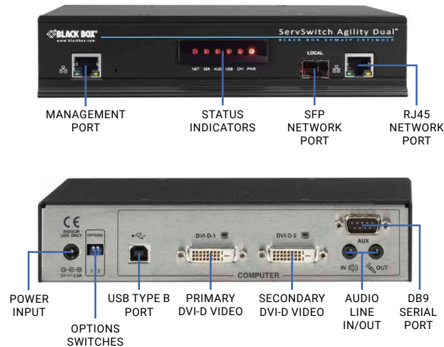
Agility Dual Head/Dual Link Transmitter (ACR1002A-T)
