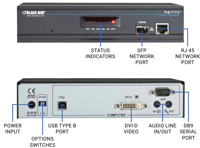
Agility Single Head Transmitter (ACR1000A-T-R2)
