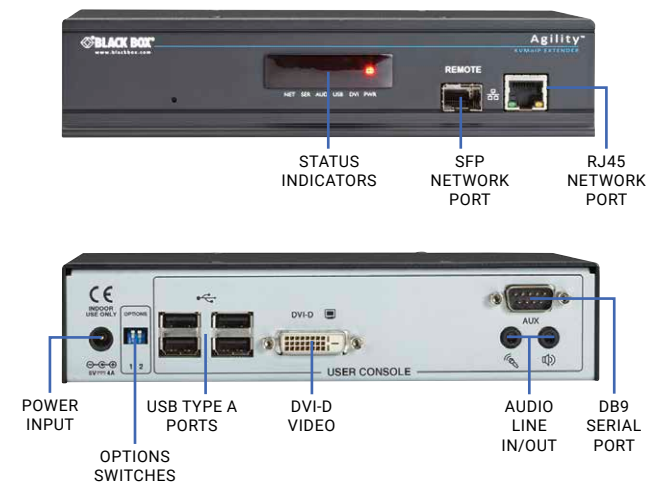
Agility Single Head Receiver (ACR1000A-R-R2)
