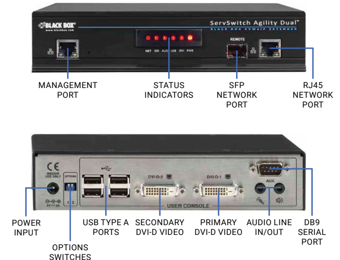
Agility Dual Head/Dual Link Receiver (ACR1002A-R)
