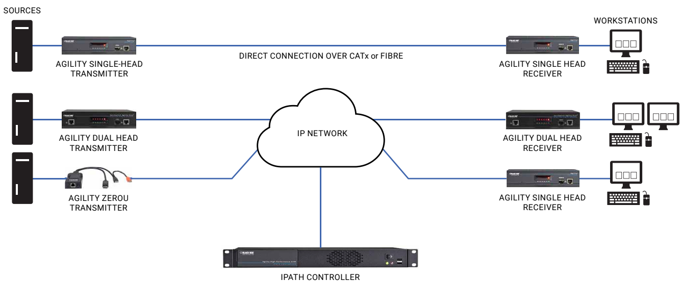
Agility point-to-point and matrix switching setup that connects multiple source PCs and user workstations.
