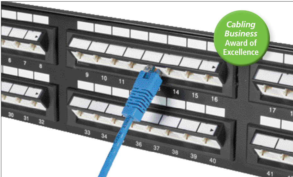
45° angled ports allow for patch cables to drape down, freeing up to 4" of cabinet depth. You'll also save time and money by eliminating horizontal cable managers in front of the panel. Shown: JPM648-45ANG
